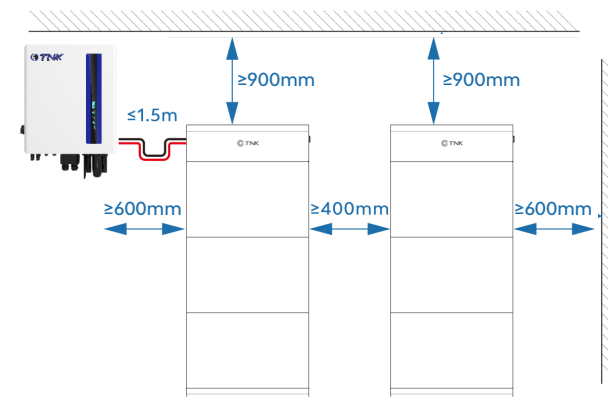
Figure 4-1 Installation space (AU/NZ region only)
