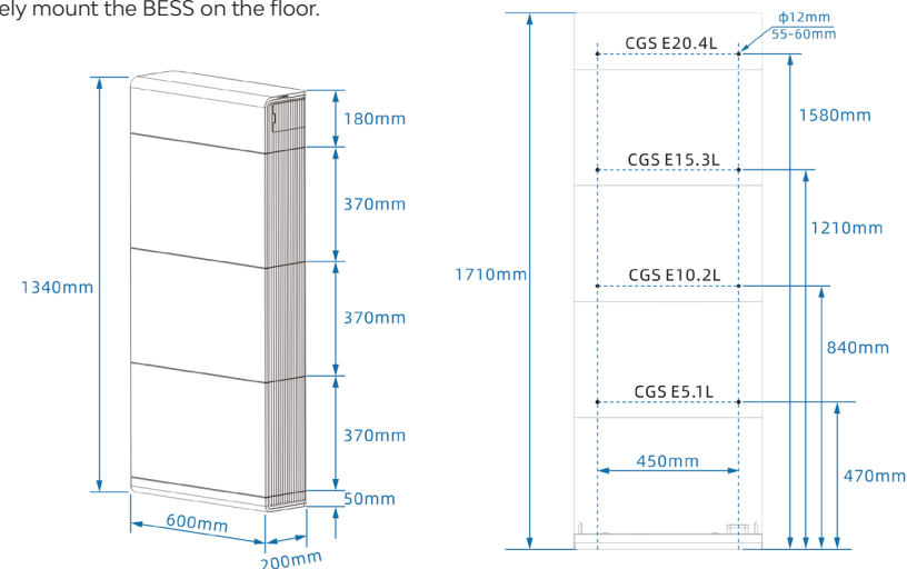
Figure 4-3 Dimensions for Floor Mounting
