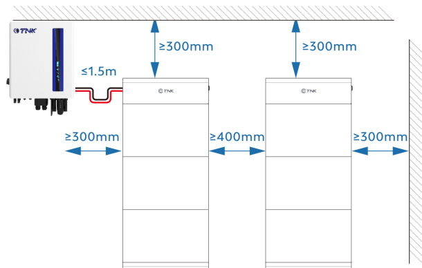
Figure 4-2 Installation Space (Other Regions)
