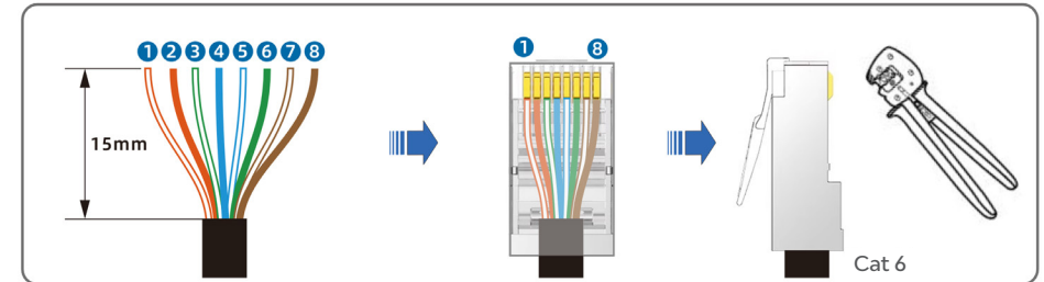
Figure 5-3 Signal Cable Preparation
