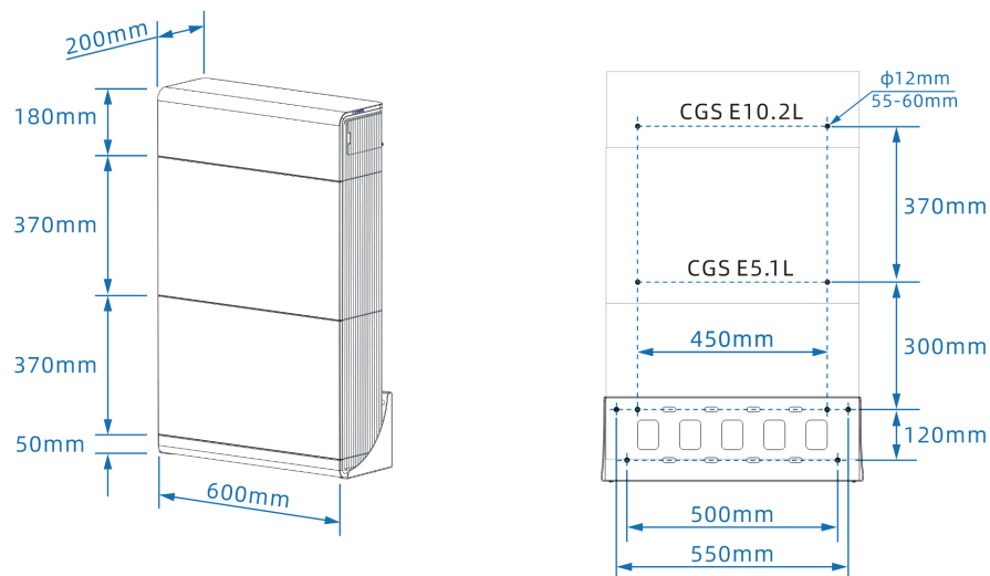
Figure 4-6 Dimensions for Wall Mounting
