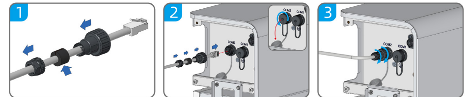
Figure 5-4 Signal Port Connections
