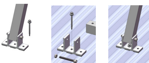
Figure 8 (Preassembly Rear Leg Installation with Single Screw)
