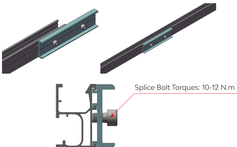
ECO-rail Installation
