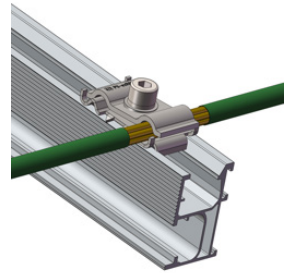
Figure 32b Installed in channel two
